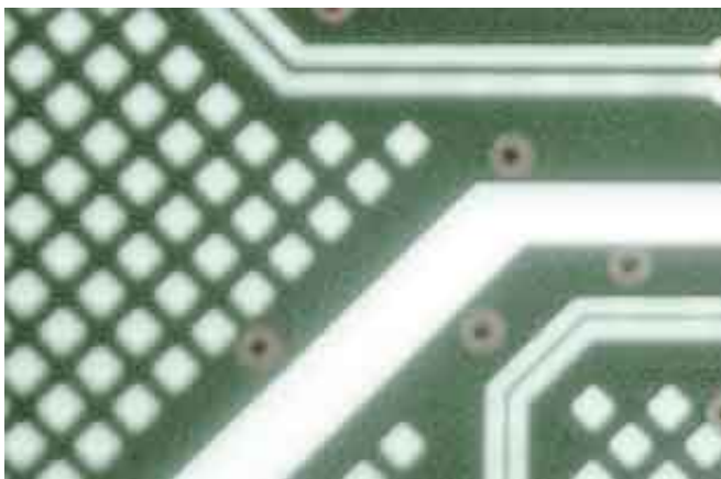
Texturepacker Pro
